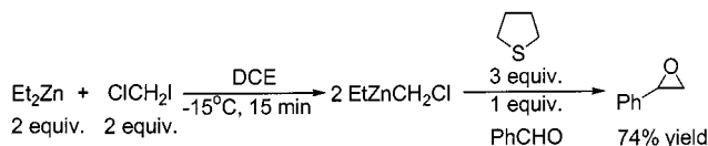
Scheme 3. Original method for epoxidation
