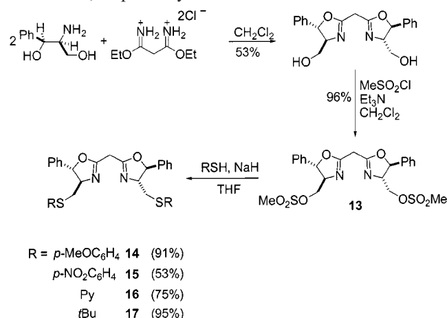
Scheme 10. Preparation of bis(oxazoline)-based sulfides
