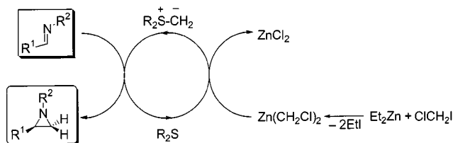
Scheme 11. Application of organozinc reagents to aziridination
