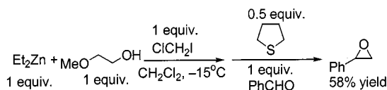
Scheme 5. Addition of chelating ligands to reduce sulfide loading
