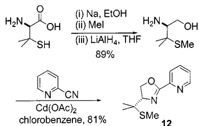
Scheme 9. Preparation of sulfide 12
