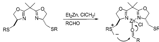
Scheme 8. Proposed reaction pathway
