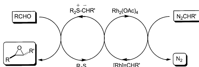
Scheme 1. Application of organorhodium reagents to epoxidation
