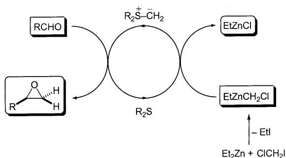
Scheme 2. Application of organozinc reagents to epoxidation
